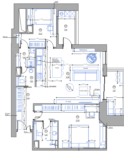
Furniture plan with dimensions
