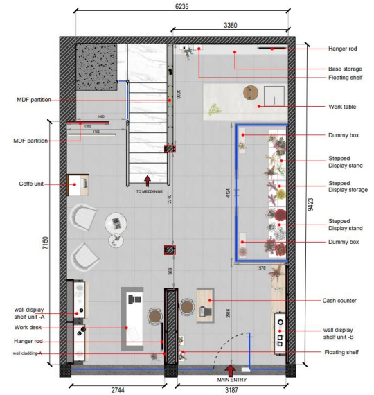
INTERIOR LAYOUT - GENERAL PLAN SCALE - NTS
